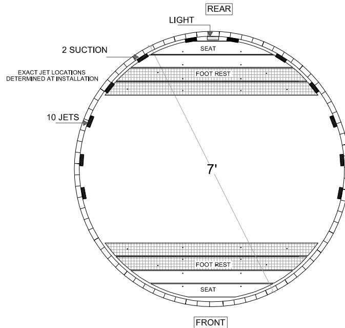
TOP PLAN
