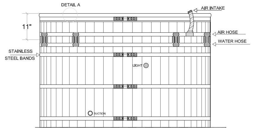
REAR ELEVATION
