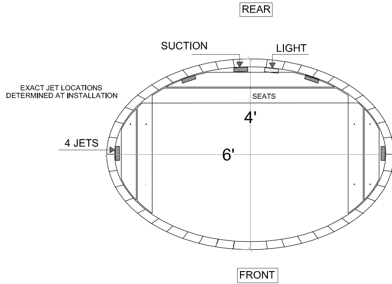
TOP PLAN
