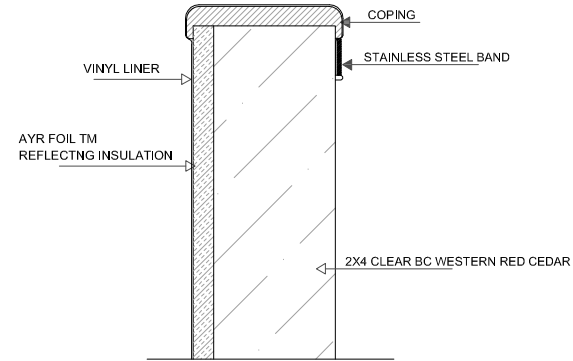
CROSS SECTION DETAIL 'A'
