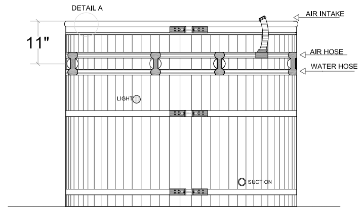
REAR ELEVATION
