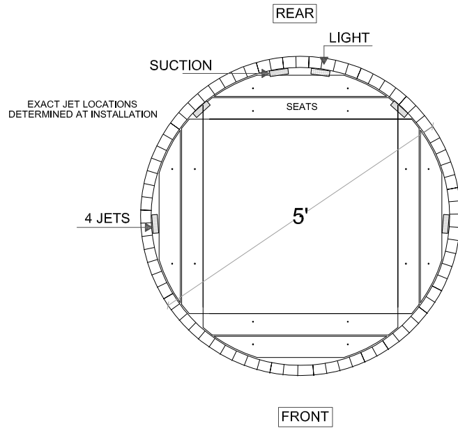
TOP PLAN
